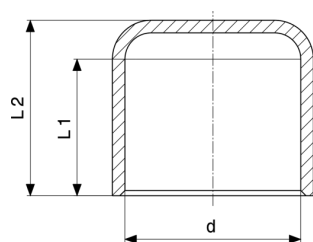
Cap - copper Model 95301
