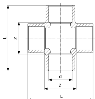
Cross piece - gunmetal Model 94180
