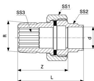
Adapter union - gunmetal, brass Model 94331G
