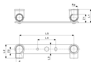
Gemini Mounting unit Model 94476.0
