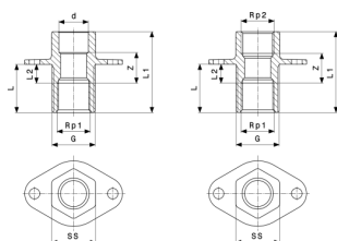
Wall lead-in - gunmetal Model 3427
