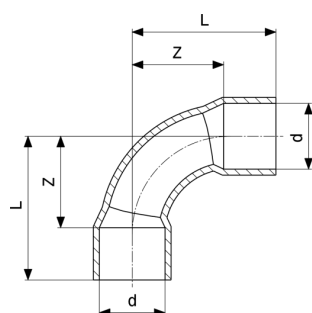
Elbow 90° - copper Model 95002A
