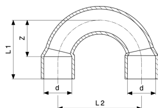
Elbow 180° - copper Model 95060
