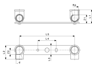
Gemini Mounting unit Model 94476.05NOR
