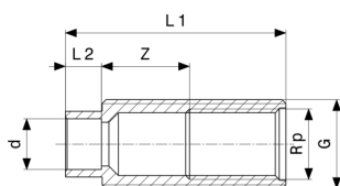
Wall lead-in - gunmetal Model 3427.2
