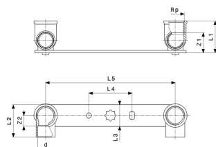
Gemini Mounting unit Model 94476.05
