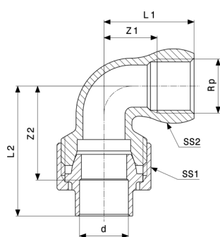
Adapter union 90° - gunmetal or silicon bronze, brass Model 94096G
